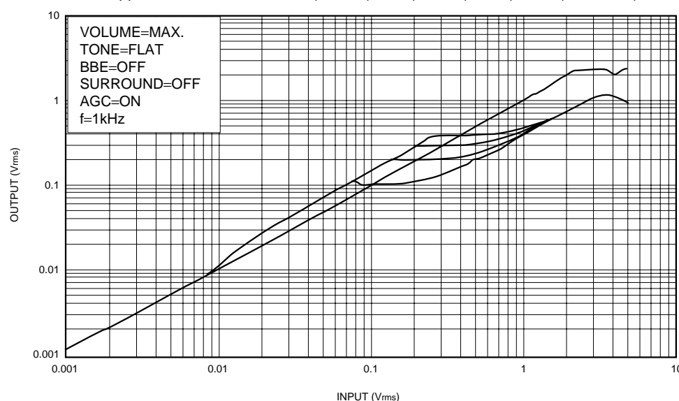
Fig.2 AGC characteristics
