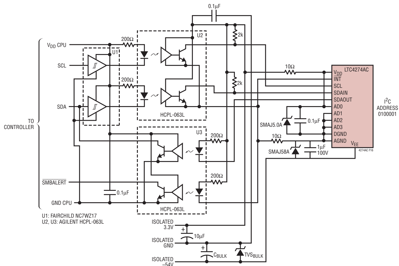
Figure 16. Opto-Isolating the I 2 C Bus
