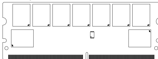
Figure 1: 244-Pin Mini-UDIMM (MO-244 R/C B)
