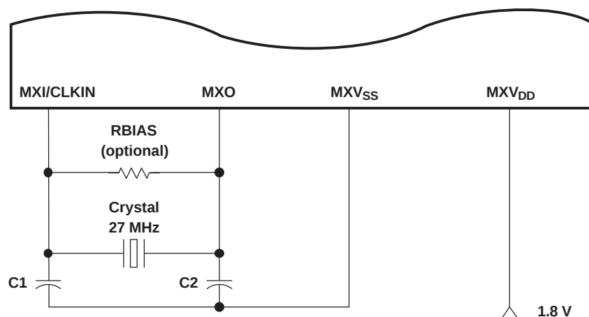
Figure 6-10. 27-MHz System Oscillator
