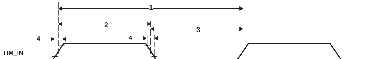
Figure 6-71. Timer Timing
