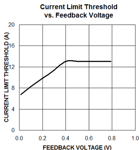
Figure 2.7 ZSPM4022-09 Current-Limit Foldback Characteristic
