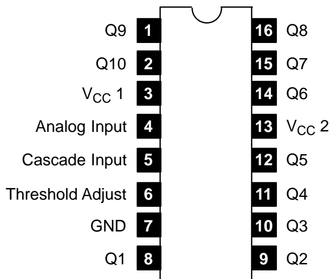
Pin Connection Diagram
