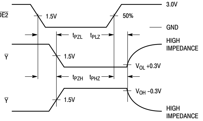
Figure 4. Switching Waveform
