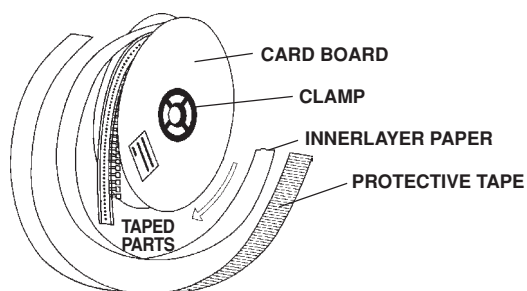
REEL PACKING
