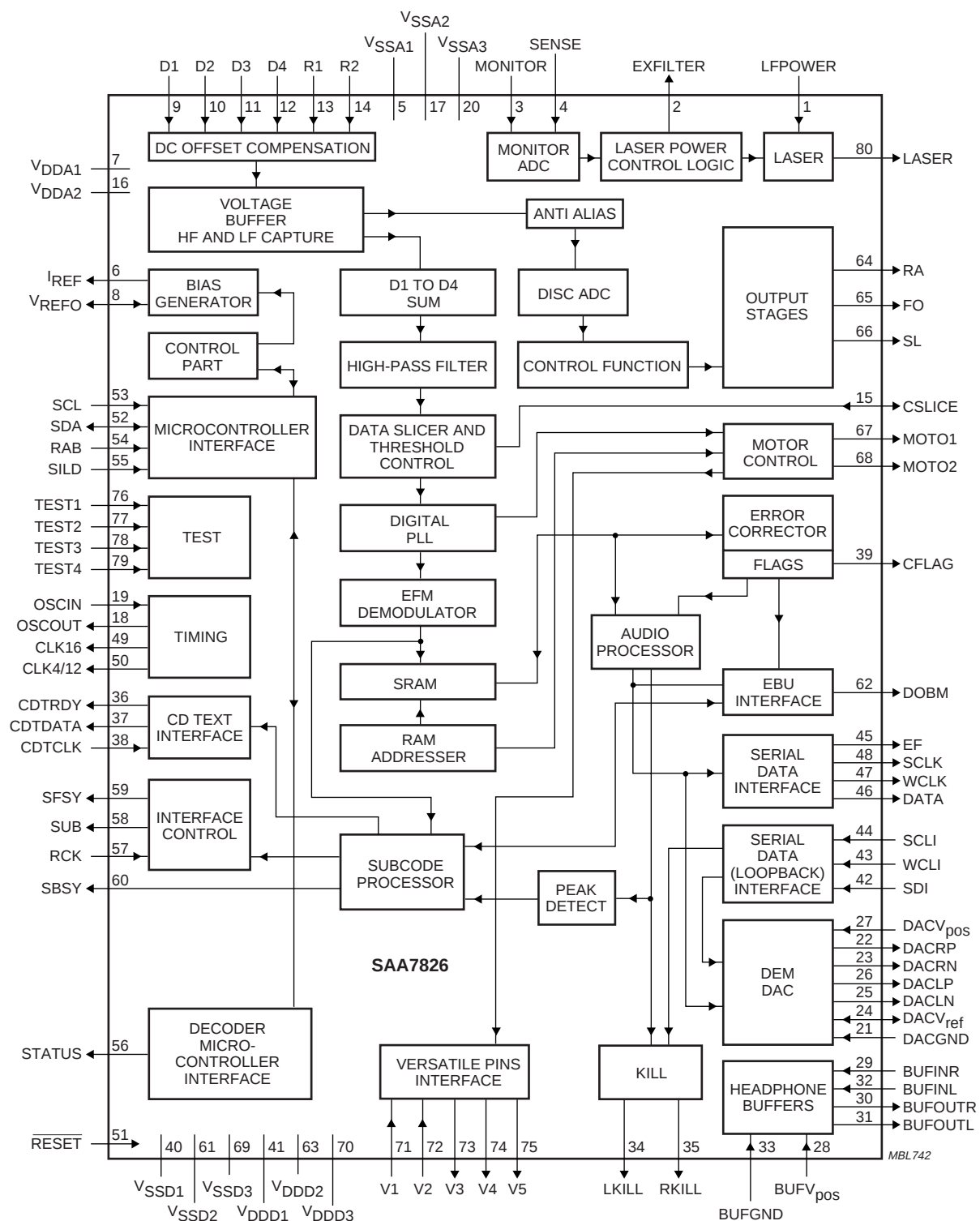
Fig.1 Block diagram.
