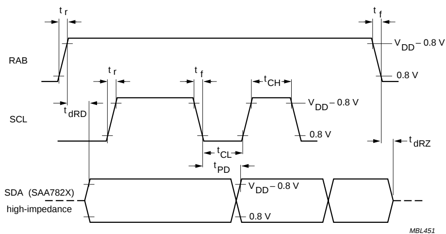
Fig.36 4-wire microcontroller timing; read mode (Q-channel subcode and decoder status information).
