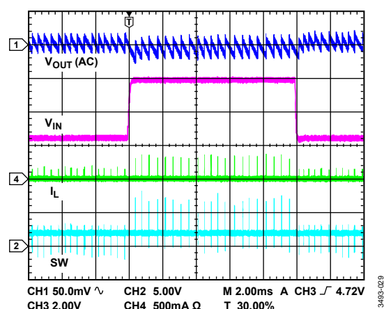
Figure 20. Line Transient, I_{LOAD} = 10 \mu A
