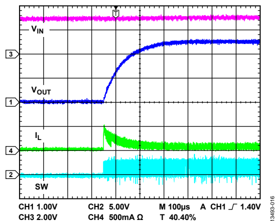
Figure 16. Soft Start, I_{LOAD} = 50 mA
