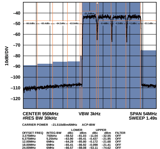
Figure 53. High Band Narrow-Band ACLR (Worse Side)
