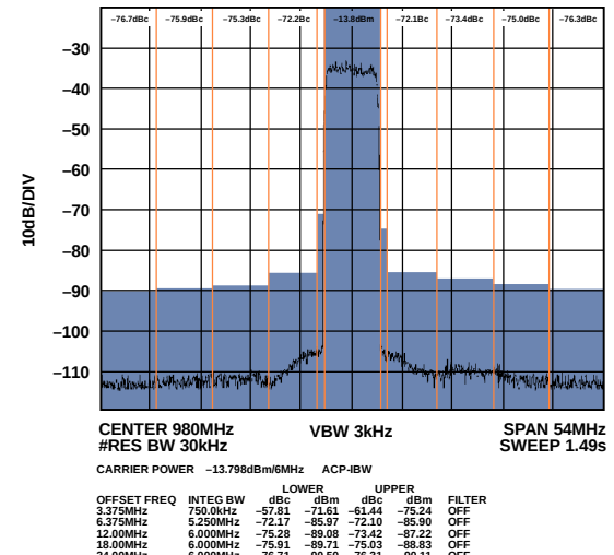
Figure 121. High Band Narrow-Band ACLR
