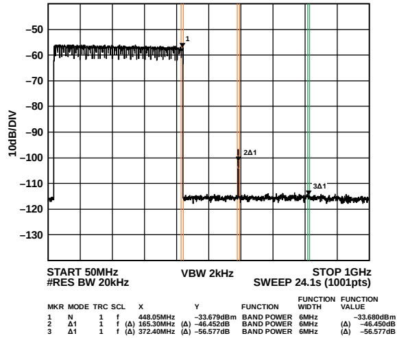
Figure 72. Low Band Wideband ACLR
