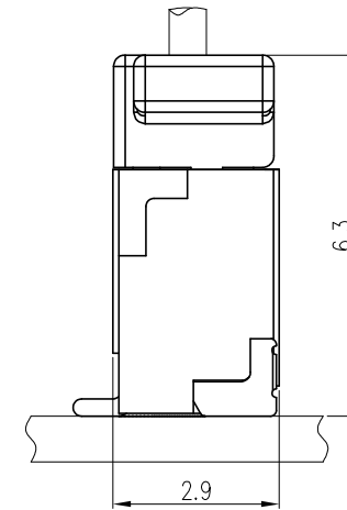
ASSEMBLY LAYOUT TOP ENTRY TYPE
