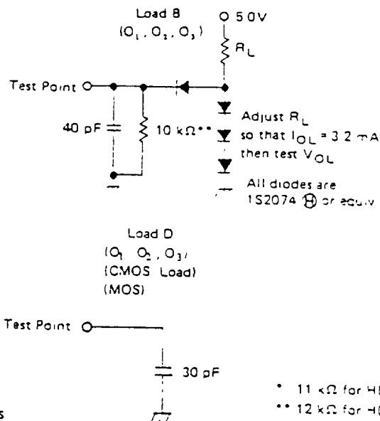
Figure 8 Test Loads
