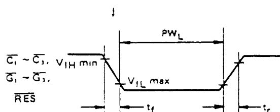
Figure 3 Input Pulse Width "Low"
