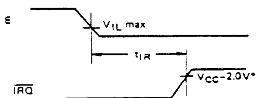
Figure 7 \overline{\text{IRQ}} Release Time
