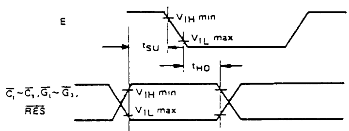
Figure 5 Input Setup and Hold Times
