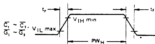
Figure 4 Input Pulse Width "High"
