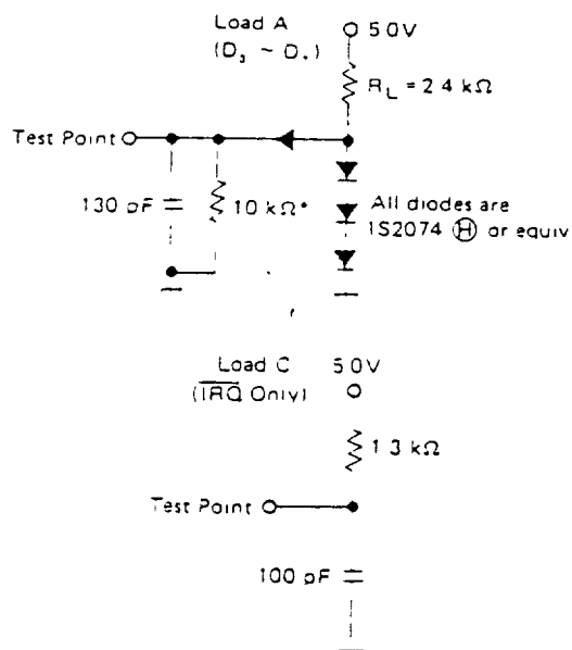
Figure 8 Test Loads
