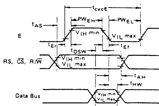
Figure 2 Bus Write Timing (Write Information into PTM)
