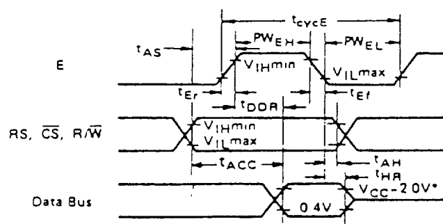
Figure 1 Bus Read Timing (Read Information from PTM)
