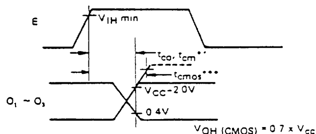
Figure 6 Output Delay
