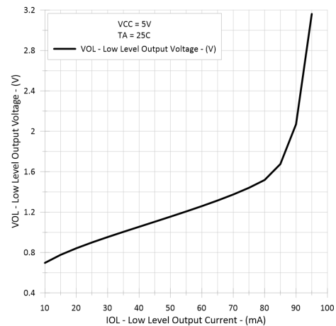
Figure 5-2. Driver Low-Level Output Voltage vs Low-Level Output Current
