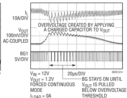
Overvoltage Protection
