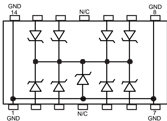
CIRCUIT DIAGRAM* - top view
