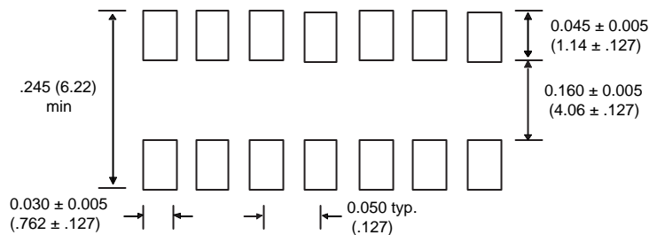
SOLDER PAD GEOMETRY
