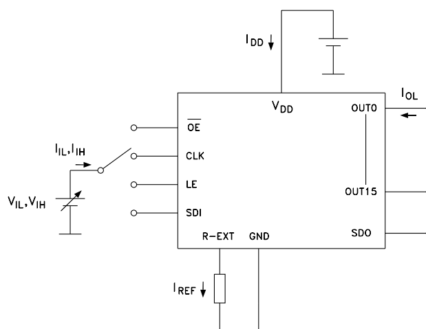
Figure 8. Typical test circuit for electrical characteristics
