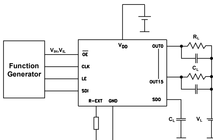
Figure 9. Typical test circuit for switching characteristics
