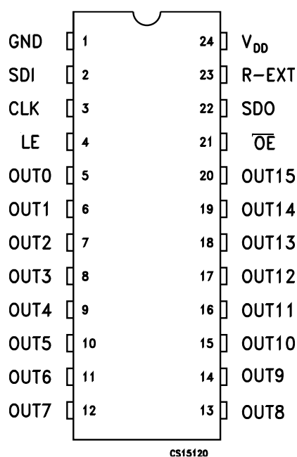
Figure 1. Pin connection
