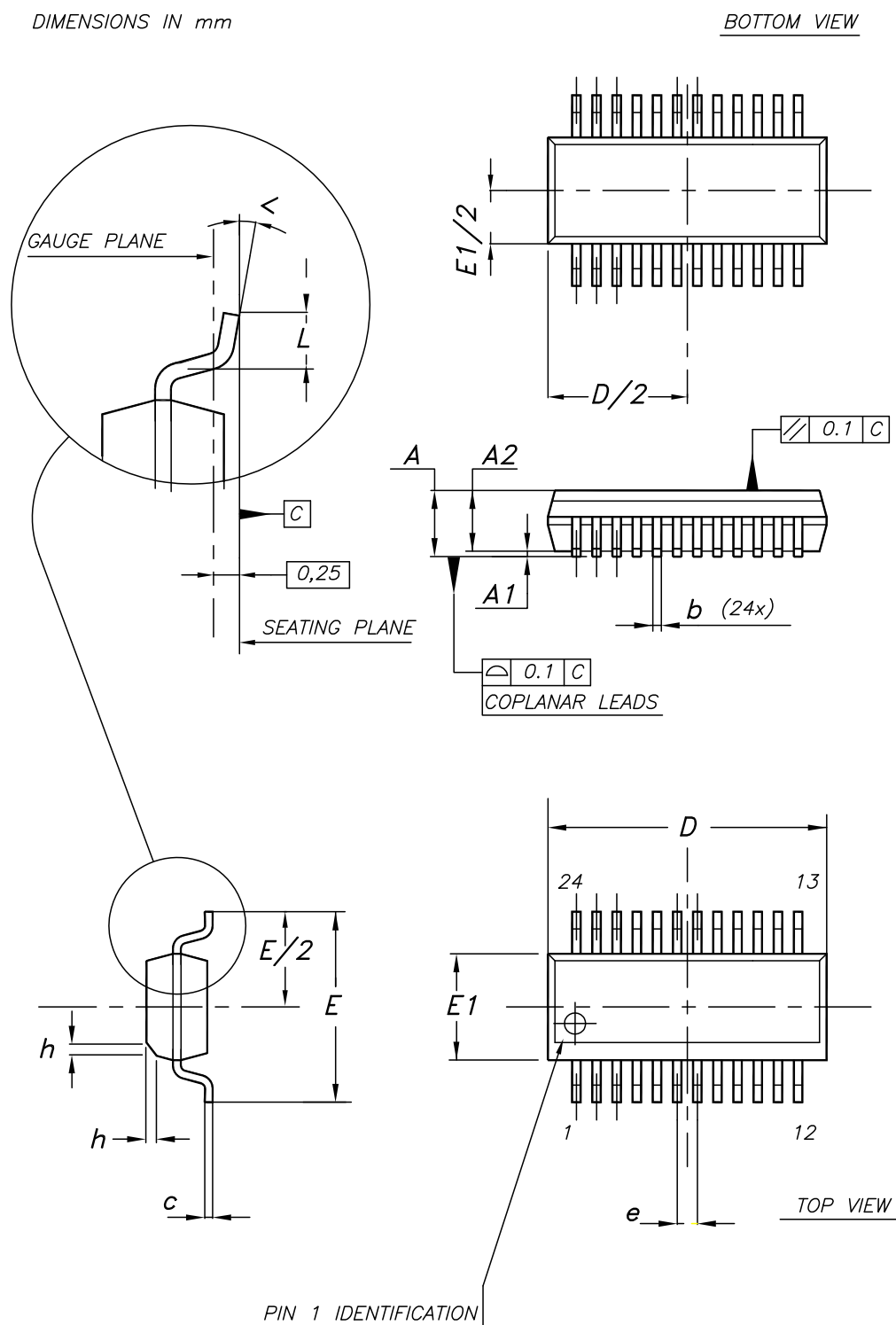
Figure 17. QSOP-24 package outline
