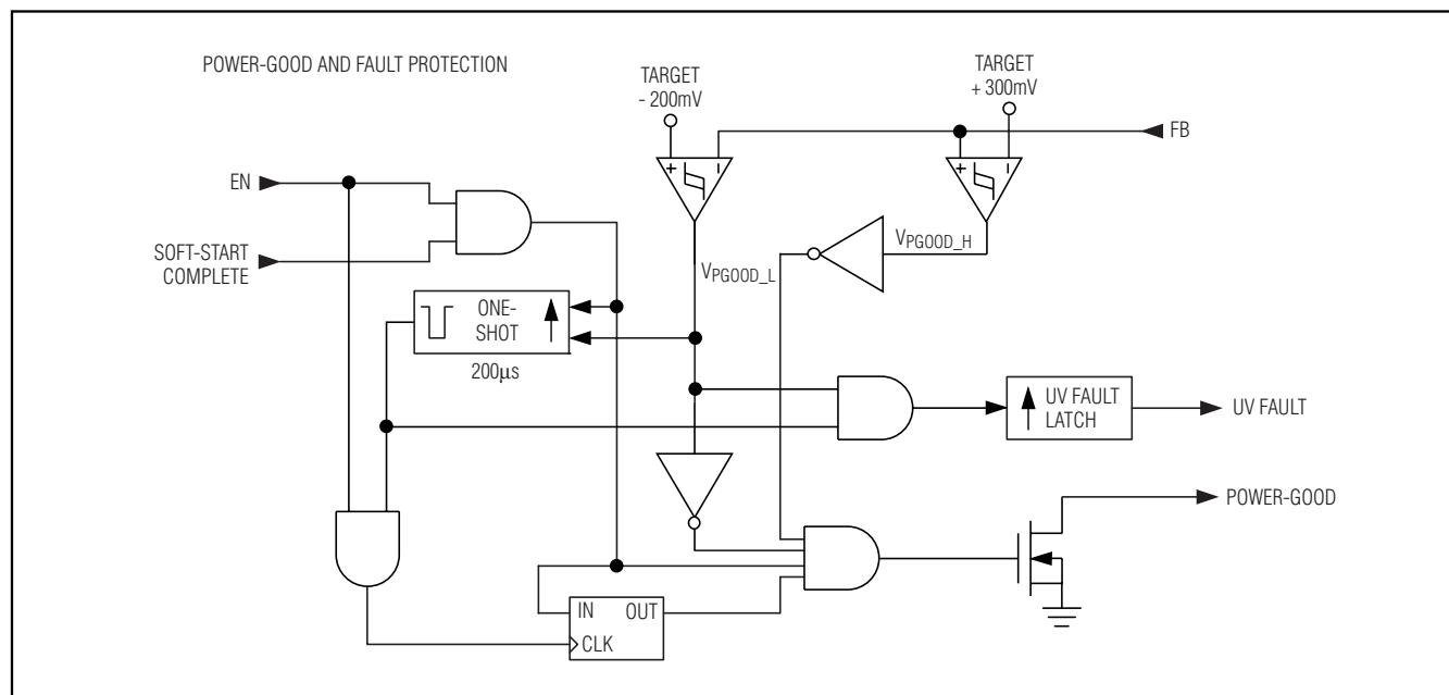
Figure 4. Power-Good and Fault Protection
