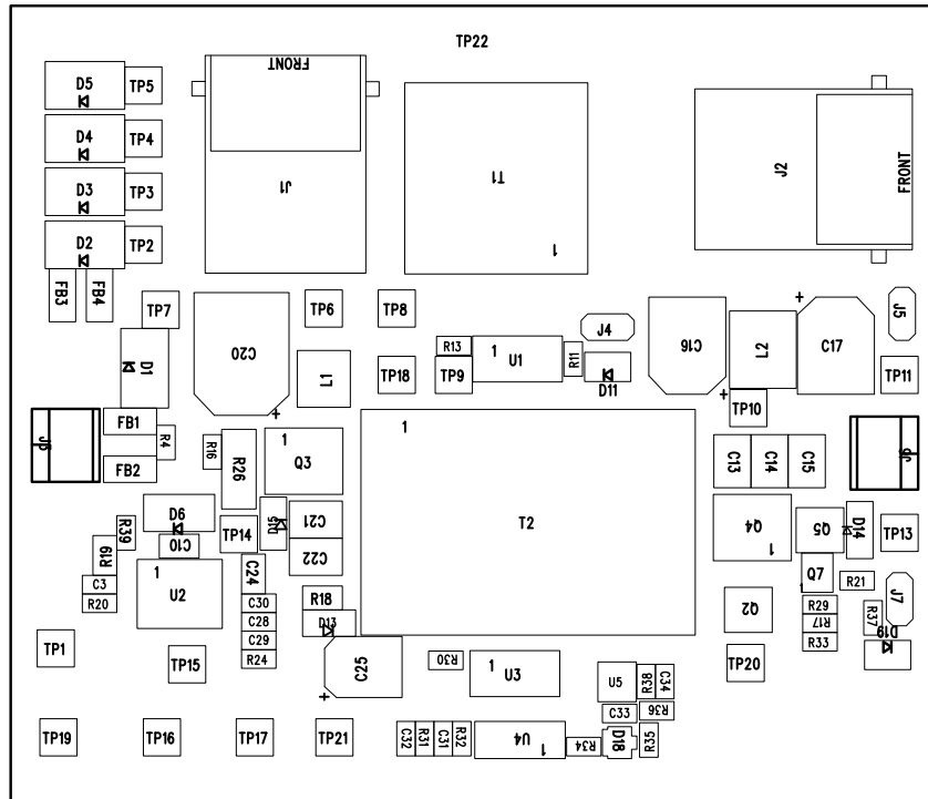
Figure 7. Top-Side Placement
