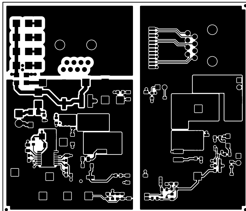
Figure 8. Top-Side Routing
