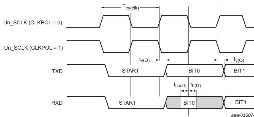
Fig 37. USART timing
