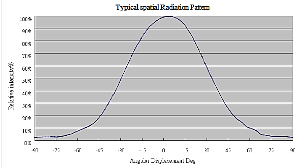
Fig. (60° Lens) Typical Representative Spatial Radiation Pattern
