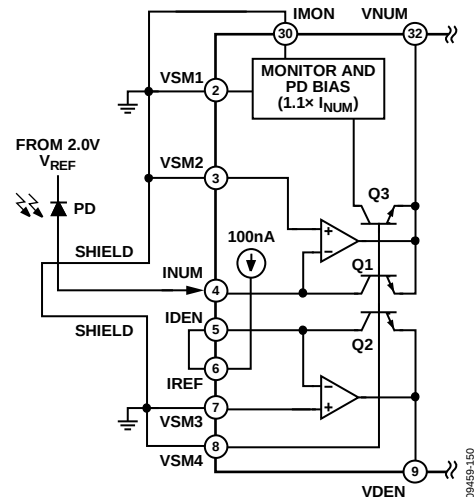
Figure 50. PD Bias with V_{\text{SUM}} at Ground and Using 2.000\text{ V}
