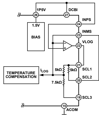
Figure 51. Buffer Amplifier in Default Configuration
