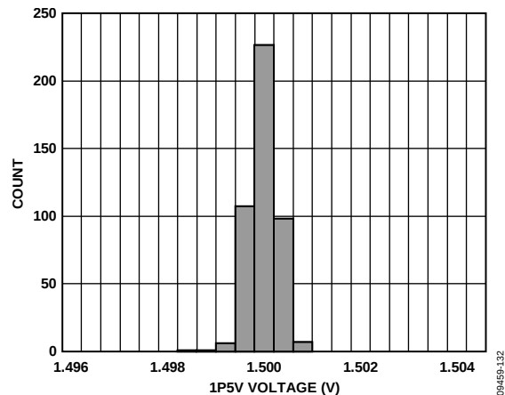
Figure 32. 1P5V Histogram
