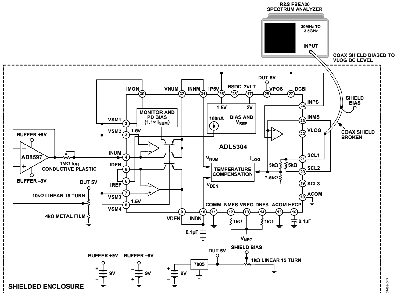
Figure 47. Setup for Measuring Noise for I_{\text{NUM}} = 100 \text{ pA} , I_{\text{NUM}} = 1 \text{ nA} , and I_{\text{NUM}} = 10 \text{ nA}
