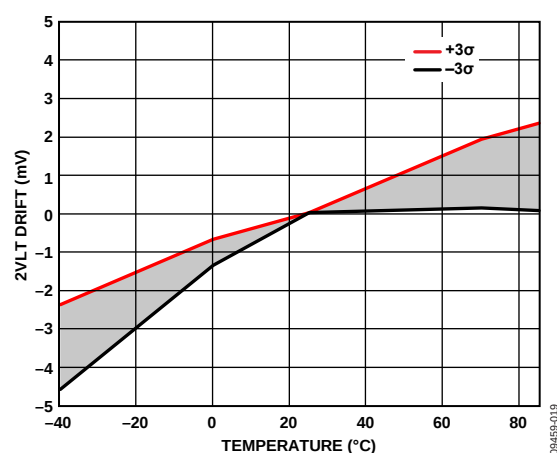
Figure 19. 2VLT Drift vs. Temperature
