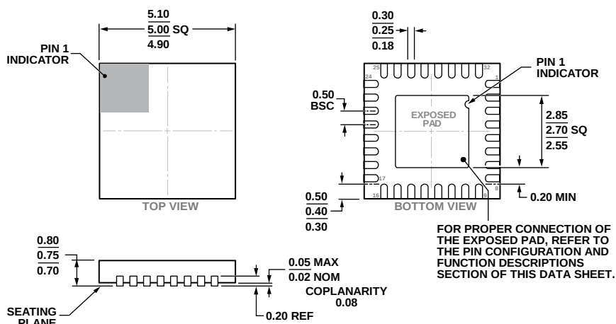
Figure 61. 32-Lead Lead Frame Chip Scale Package [LFCSP] 5 mm × 5 mm Body and 0.75 mm Package Height (CP-32-21)
