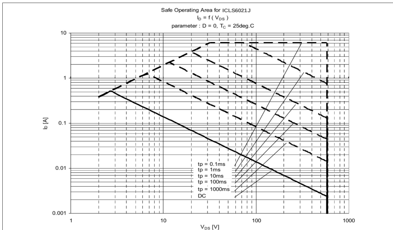
Figure 20 Safe Operating Area (SOA) curve for ICLS6023J
