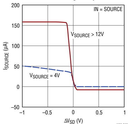
SOURCE Current vs Forward Voltage Drop
