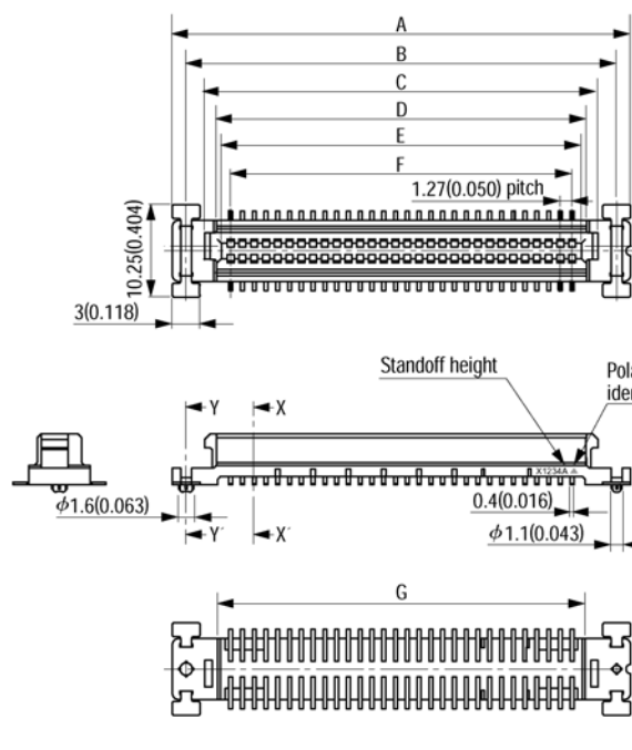
A Type (Standoff height)
