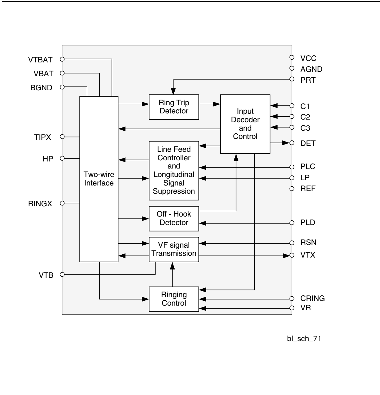
Figure 1 Block Diagram
