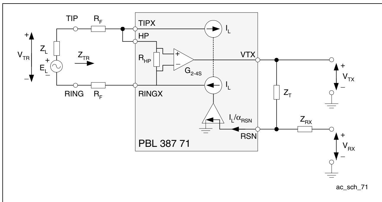
Figure 9 Simplified AC Model of PBL 38771/1
