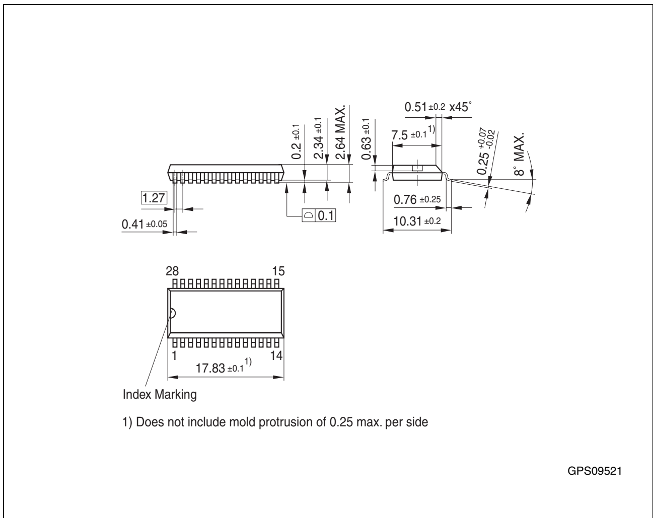
Figure 16 P-DSO-28-20 (Plastic Dual Small Outline Package)
