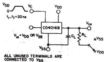
Fig. 22 - Max. control-input repetition rate.
