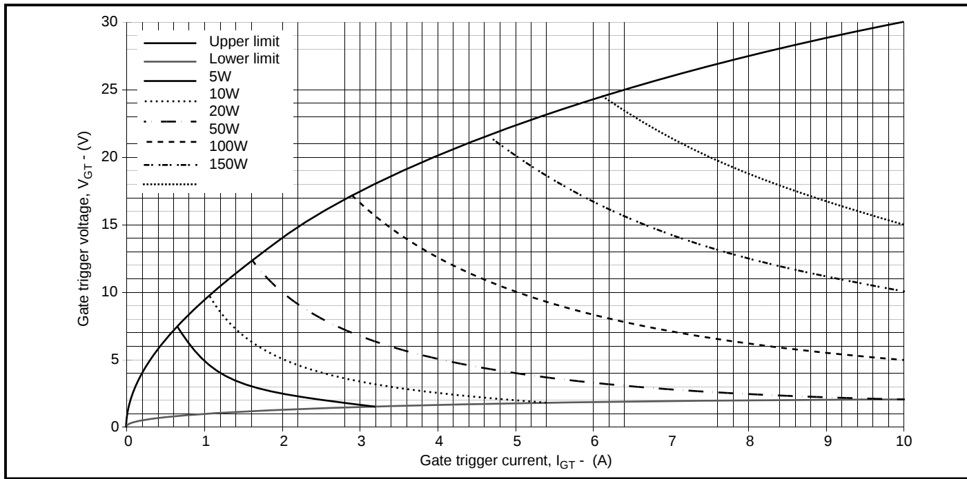
Fig.9 Gate characteristics
