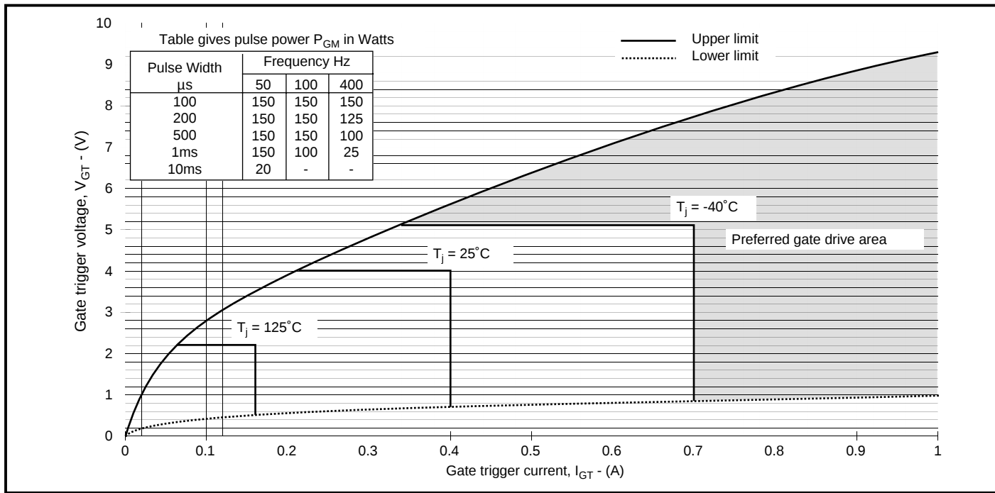
Fig.8 Gate characteristics
