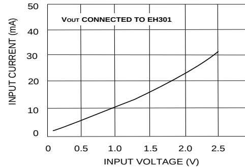
INPUT CURRENT AS A FUNCTION OF INPUT VOLTAGE
