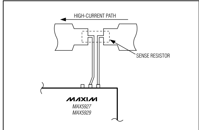
Figure 13. Kelvin Connection for the Current-Sense Resistors
