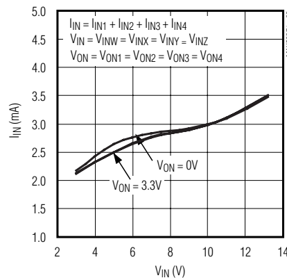
TOTAL SUPPLY CURRENT vs. INPUT VOLTAGE
