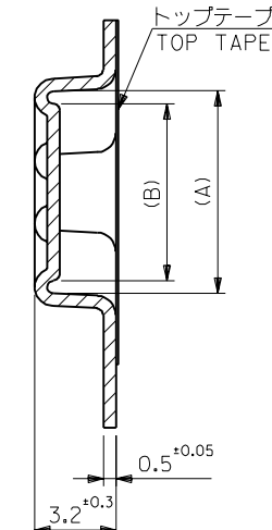
SECT:Y-Y (SCALE 5:1)
