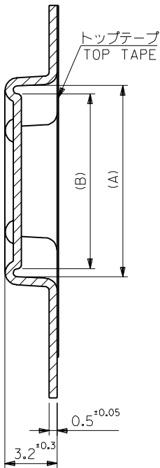
SECT:Y-Y (SCALE 5:1)
