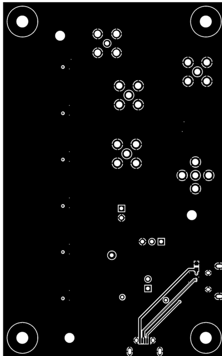
Figure 7. Bottom Layer
