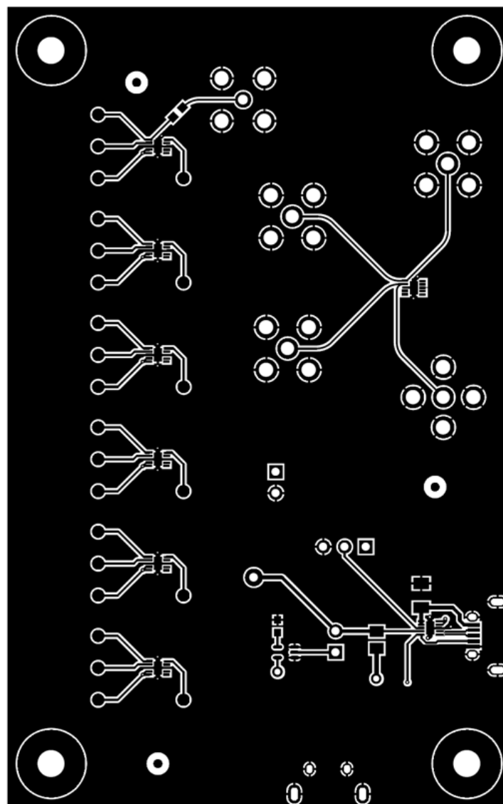
Figure 4. Top Layer
