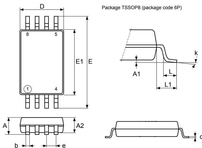
Figure 12. TSSOP8 – Outline
