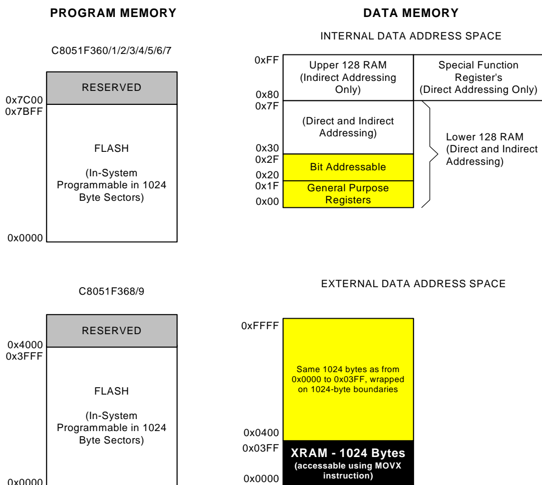
Figure 9.2. Memory Map
