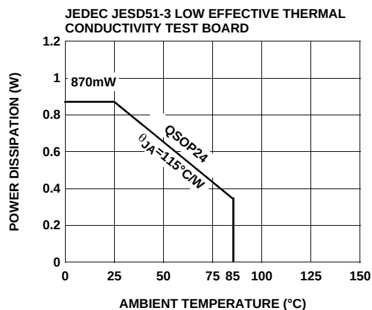
FIGURE 35. PACKAGE POWER DISSIPATION vs AMBIENT TEMPERATURE
