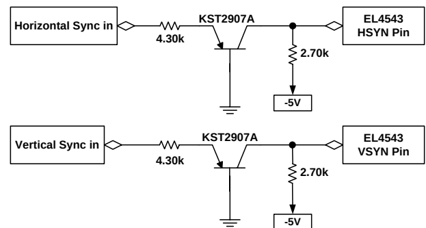
FIGURE 40. LEVEL SHIFTING SYNC SIGNALS FOR USE WITH ±5V SPLIT RAILS
