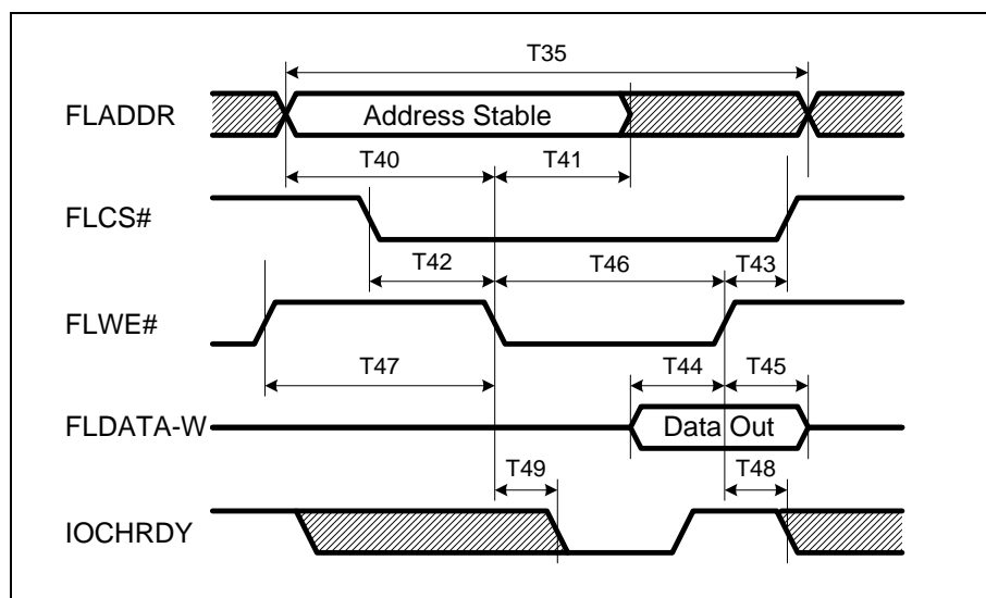
Figure 27. Flash/Modem Timings for a Write Cycle
