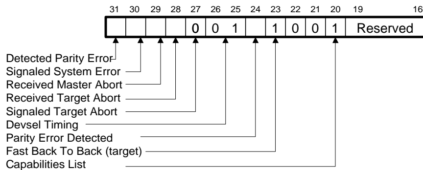
Figure 17. PCI Status Register
