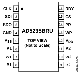
Figure 4. Pin Configuration
