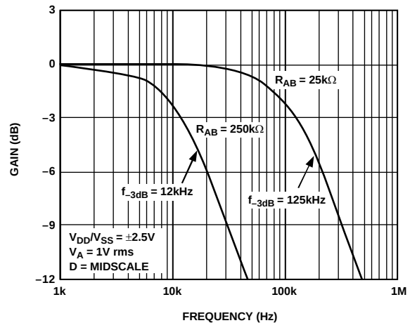
Figure 15. -3\text{ dB} Bandwidth vs. Resistance (Figure 31)
