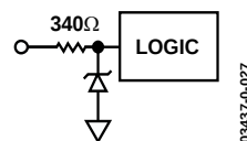
Figure 28. ESD Protection of Digital Pins
