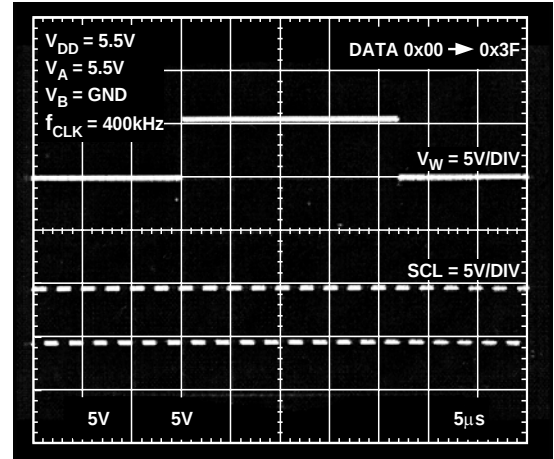
Figure 20. Settling Time
