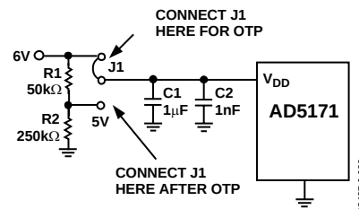
Figure 25. Power Supply Requirement
