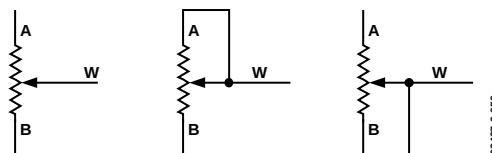
Figure 30. Rheostat Mode Configuration
