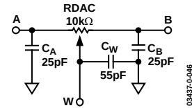
Figure 47. Circuit Simulation Model for RDAC = 10 k \Omega
