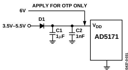
Figure 26. Isolating the 6 V OTP Supply from the 3.5 V to 5.5 V Normal Operating Supply. The 6 V supply must be removed once OTP is complete.
