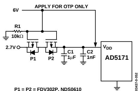
Figure 27. Isolating the 6 V OTP Supply from the 2.7 V Normal Operating Supply. The 6 V supply must be removed once OTP is complete.
