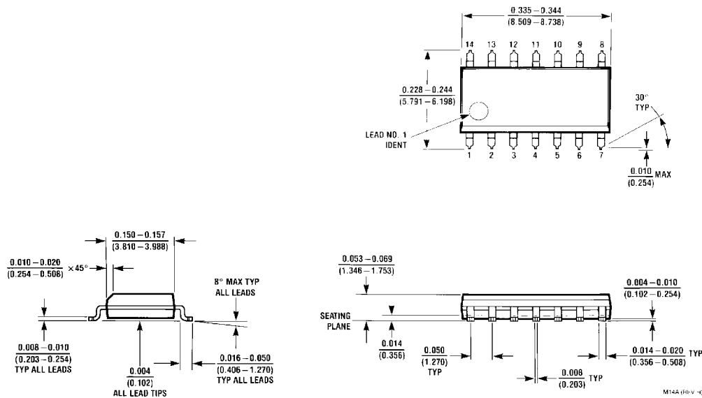
S.O. Package (M) Order Number DM74ALS32M Package Number M14A
