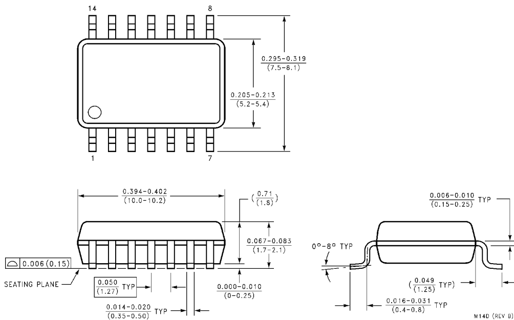
Small Outline Package (SJ) Order Number DM74ALS32SJ Package Number M14D
