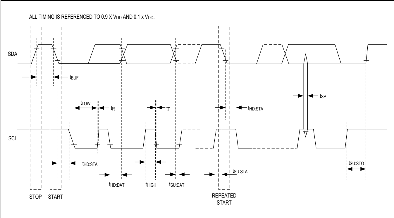
Figure 3. Timing Diagram
