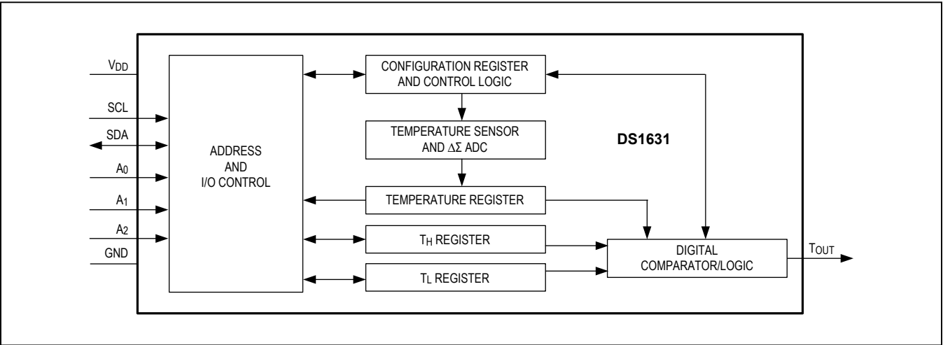
Figure 1. Functional Diagram
