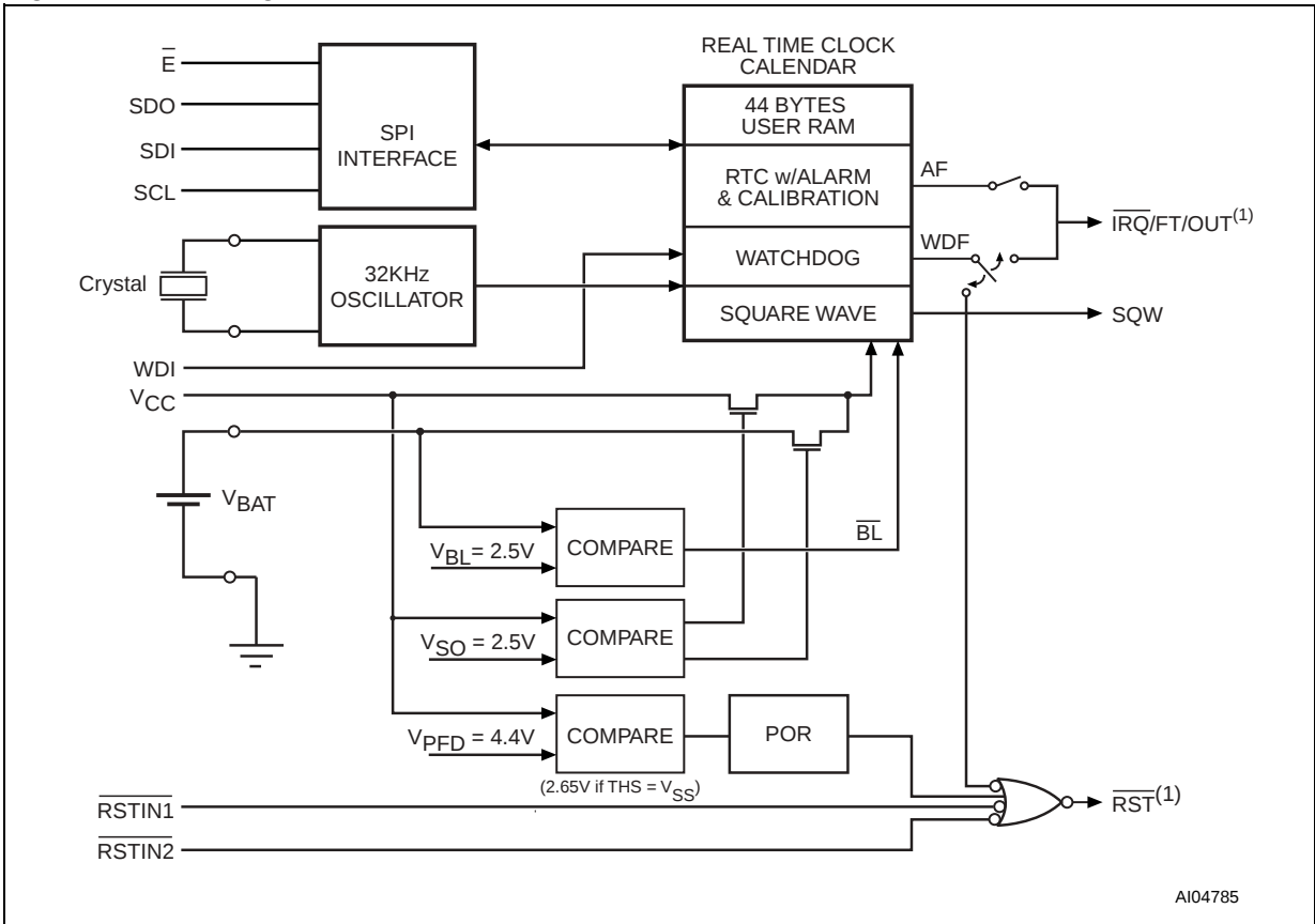
Figure 6. Block Diagram
