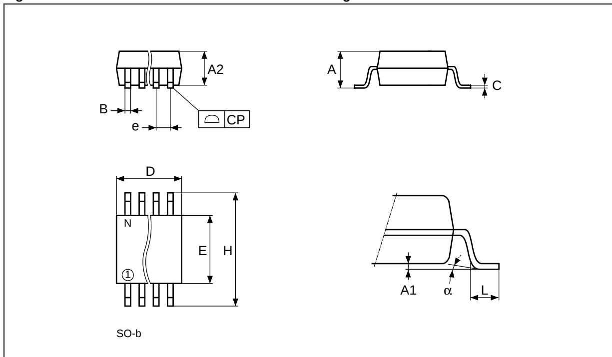
Figure 20. SO16 – 16-lead Plastic Small Outline Package Outline
