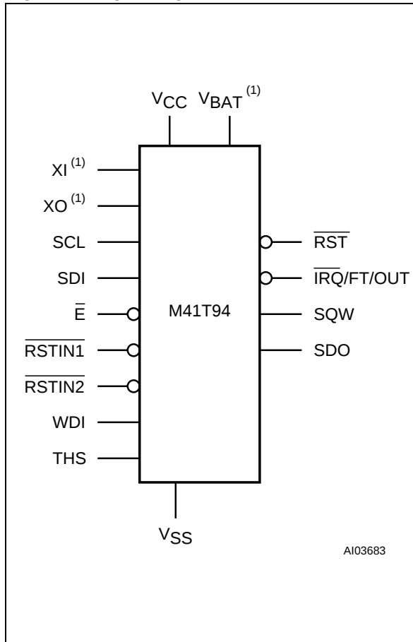
Figure 3. Logic Diagram
