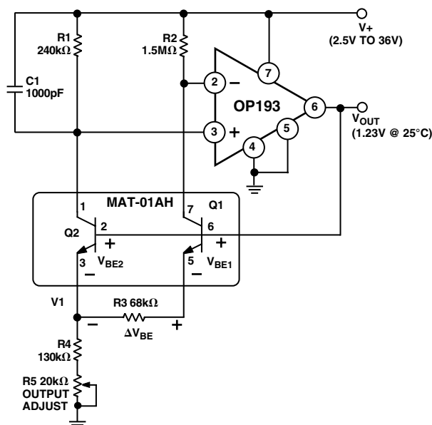
Figure 7. A Battery-Powered Voltage Reference
