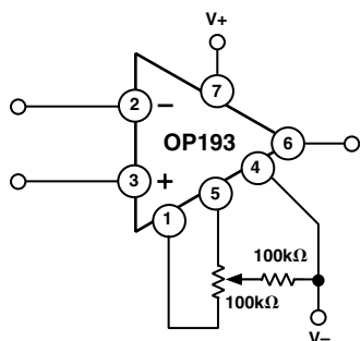
Figure 5. High Resolution Offset Nulling Circuit
