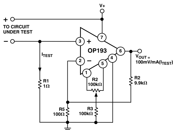
Figure 8. Single-Supply Current Monitor
