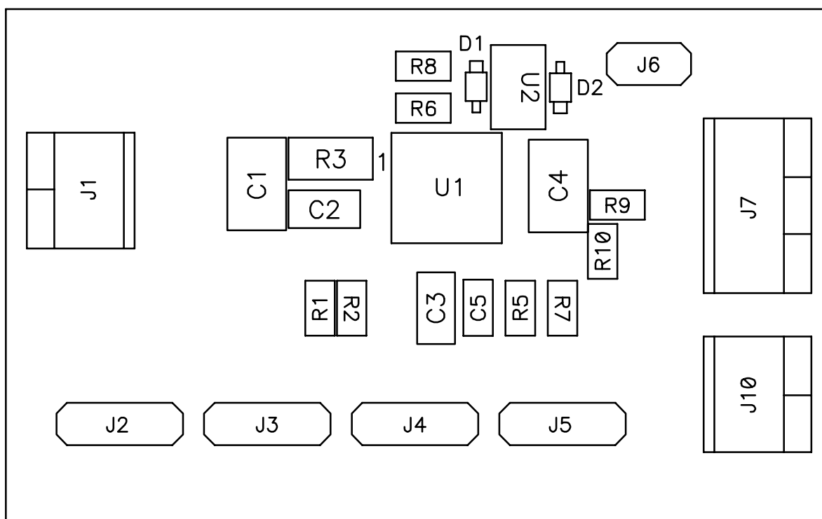
Figure 3–3. SLUP167 Top Assembly View
