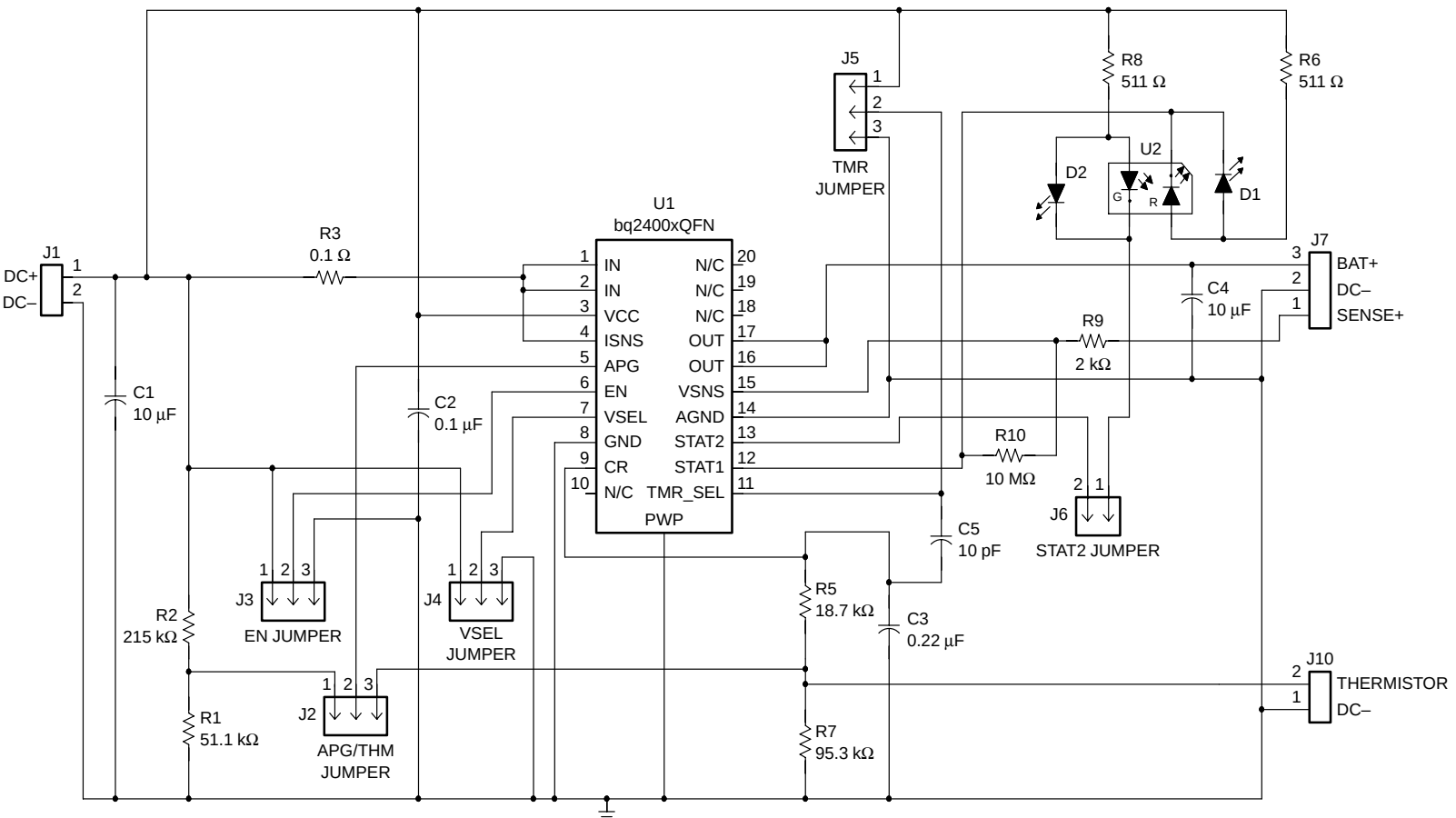
Figure A-1 shows the bq24001 EVM (SLUP167) schematic diagram.
