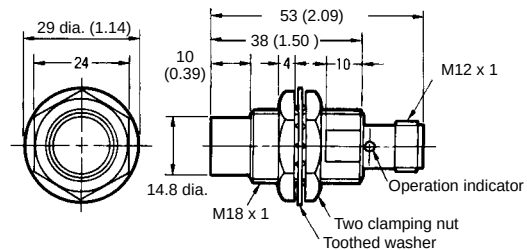
Fig.17: E2E-X10ME□-M1/F□-M1-N
