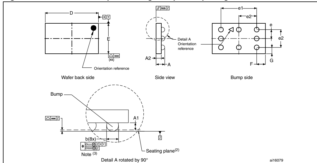
Figure 22. WLCSP – 8 bump wafer length chip scale package
