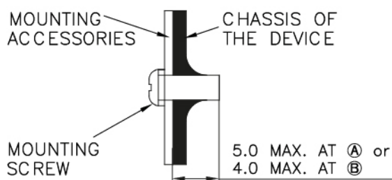
Fig. 4 Assembly Reference
