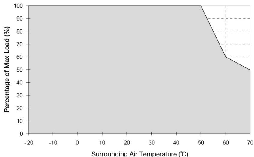
Fig. 1 De-rating for Vertical and Horizontal Mounting Orientation > 50°C de-rate power by 4% / °C > 60°C de-rate power by 1% / °C
