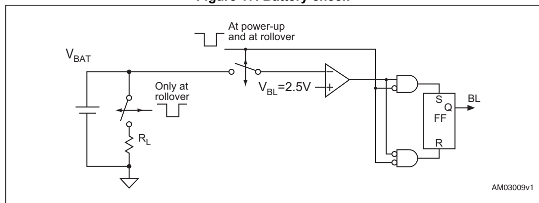
Figure 17. Battery check
