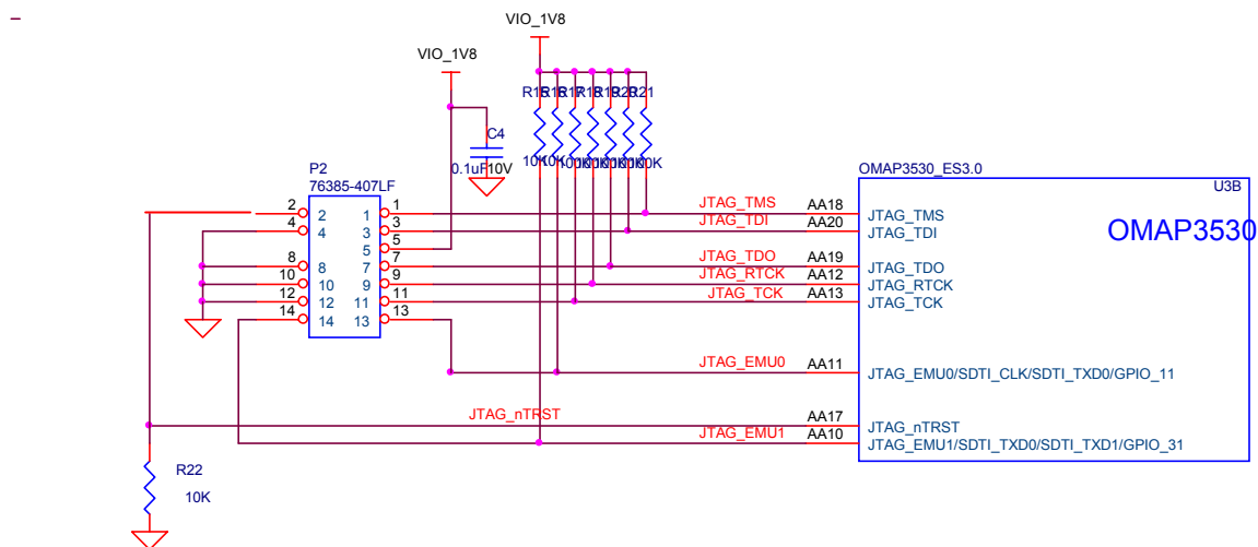
Figure 45. JTAG Interface
