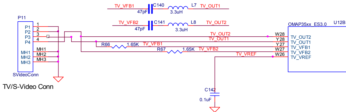
Figure 41. S-Video Interface
