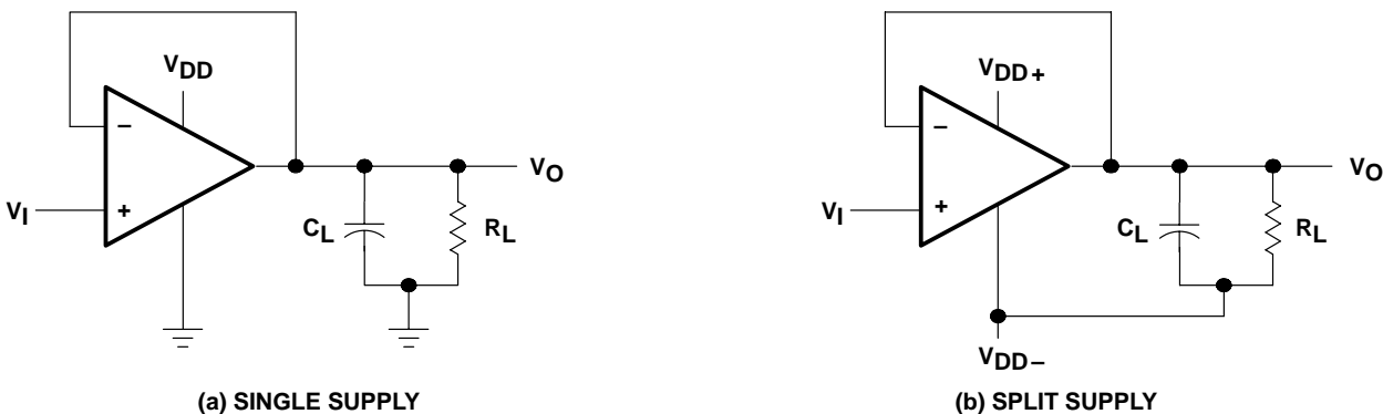
Figure 33. Unity-Gain Amplifier
