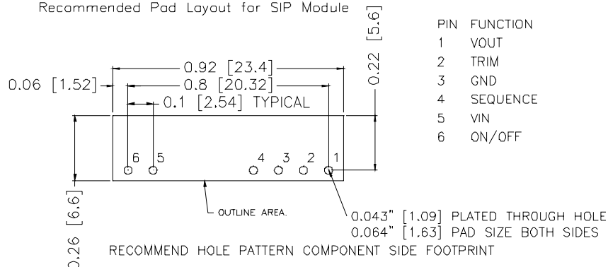
Recommended Pad Layout for SIP Module
